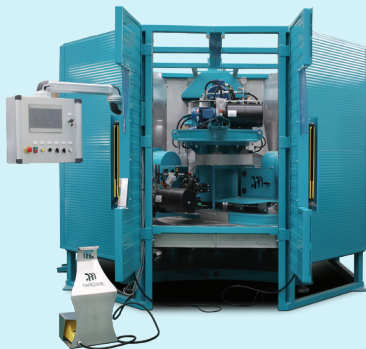
Complementary Wrecker and Extractor machines
