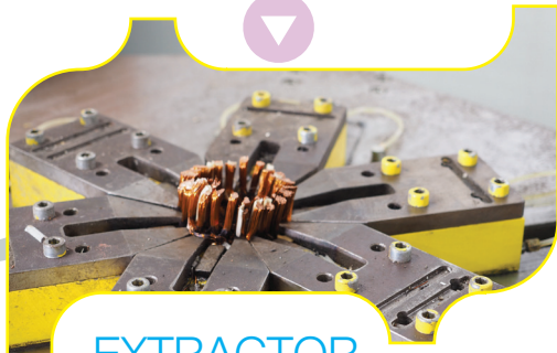
EXTRACTOR MACHINE
